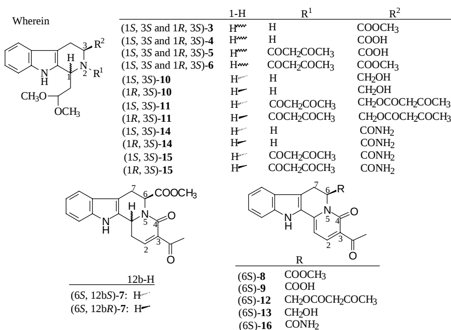
Scheme 1 The synthesis route for enantiopure oxoindolo-quinolizines
